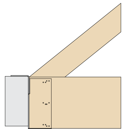
Plates omitted for clarity Minimum bottom chord depth or vertical required for trusses
