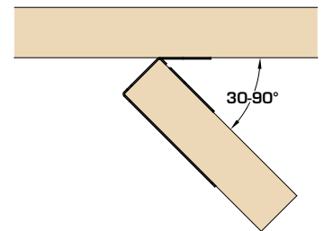
Left hand skew (skews between 30–90°)
