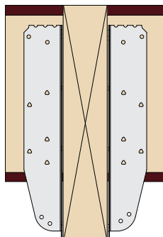
UH OR HUH* – 235MM DEEP (235–254mm deep joists)
