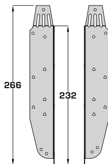
UH-235 (To suit 235 – 245mm deep i-joists)
