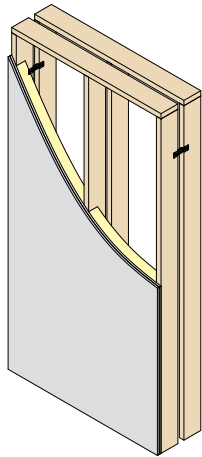
E-WT-1 (timber frame cavity wall without sheathing)
