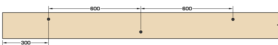
Figure 4 – Top Chords/Webs of Depths 122mm, 147mm, 172mm, 197mm or 222mm
